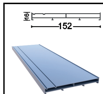
OPT-1009-50 Side Profile 5 Rails Weight 1.35 kg/m
