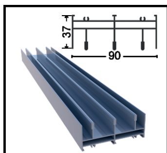
OPT-1002-60 Top Frame Profile 3 Rails Weight 1.46 kg/m
