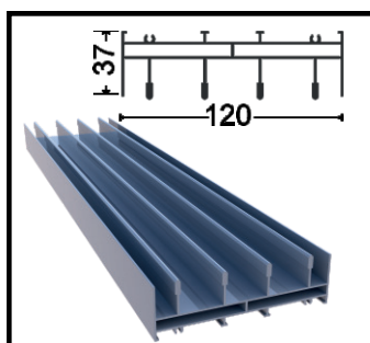
OPT-1005-60 Top Frame Profile 4 Rails Weight 1.855 kg/m
