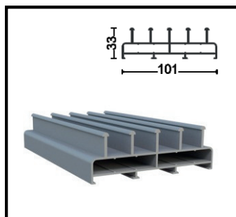
SRM-1002 Bottom Frame Profile (with Treshold) Weight 1.488 kg/m
