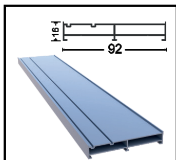
OPT-1003-50 Side Profile 3 Rails Weight 0.886 kg/m
