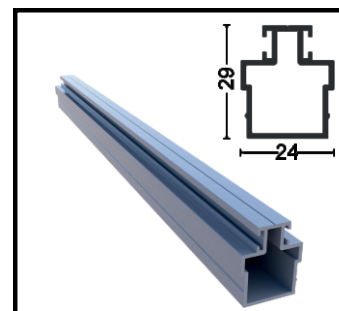
OPT-1015-50 Middle Joint Profile
