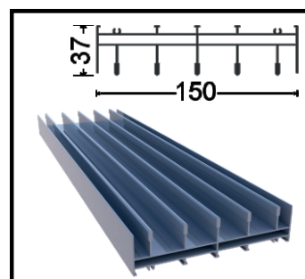
OPT-1008-60 Top Frame Profile 5 Rails Weight 2.246 kg/m
