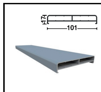
SRM-1006 Aluminum Side Post Profile Weight 0.928 kg/m
