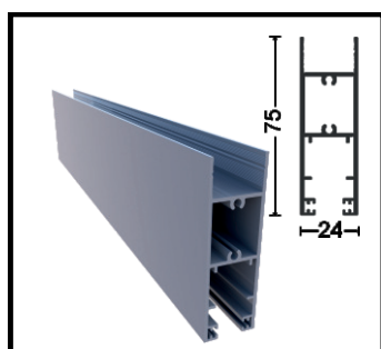
OPT-1010-60 Glass Profile Double Glazed Weight 0.968 kg/m
