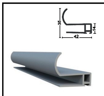
SRM-1008 End Profile Weight 0.596 kg/m
