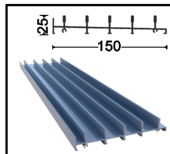
OPT-1007-60 Bottom Frame Profile 5 Rails Weight 1.68 kg/m
