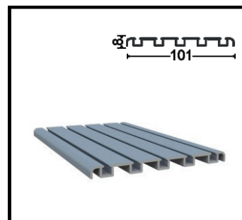
SRM-1002 Bottom Frame Profile (without Treshold) Weight 0.766 kg/m
