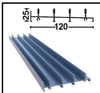
OPT-1004-60 Bottom Frame Profile 4 Rails Weight 1.37 kg/m
