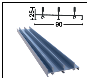
OPT-1001-60 Bottom Frame Profile 3 Rails Weight 1.06 kg/m
