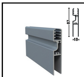
SRM-1004 Aluminum Glass Carrier Base Profile(8 mm) Weight 1.167 kg/m
