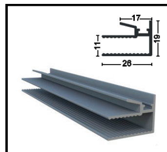
SRM-1009 Puller Profile (8 mm) Weight 0.285 kg/m
