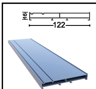
OPT-1006-50 Side Profile 4 Rails Weight 1.124 kg/m
