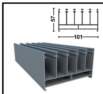
SRM-1001 Top Frame Profile Weight 2.038 kg/m
