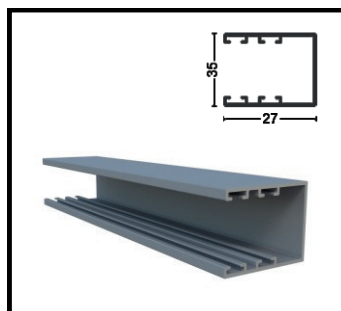
SRM-1007 "U" Profile Weight 0.395 kg/m
