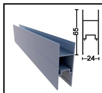
OPT-1012-50 End Profile with Espagnolette Weight 0.67 kg/m
