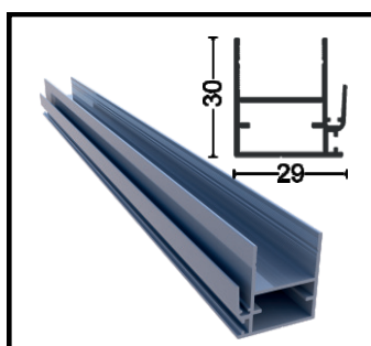
OPT-1011-50 Pull Profile Double Glazed Weight 0.434 kg/m
